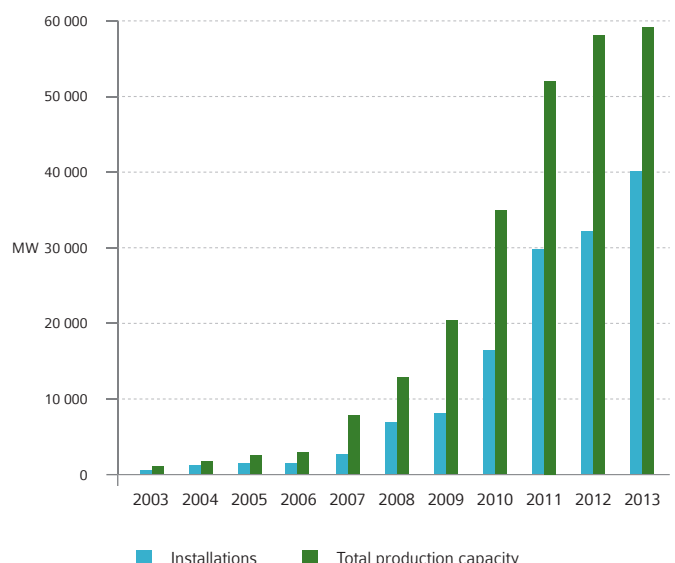
FIGURE 18: PV INSTALLATIONS AND PRODUCTION CAPACITIES (MW)
